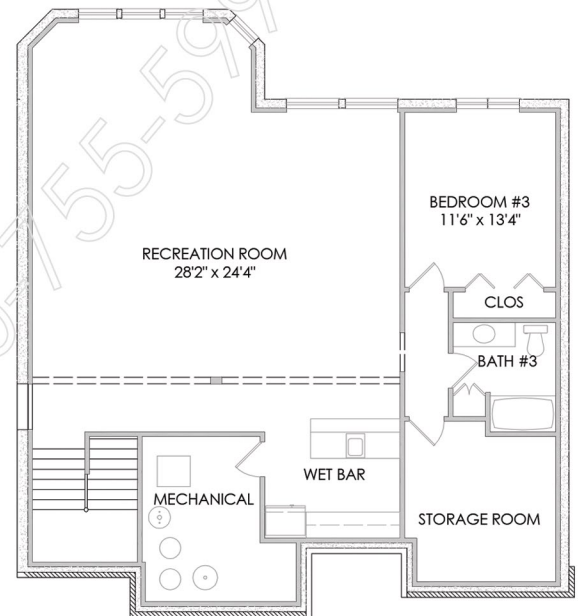
Basement (Opt.)
