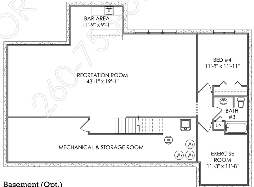
Basement (Opt.)
